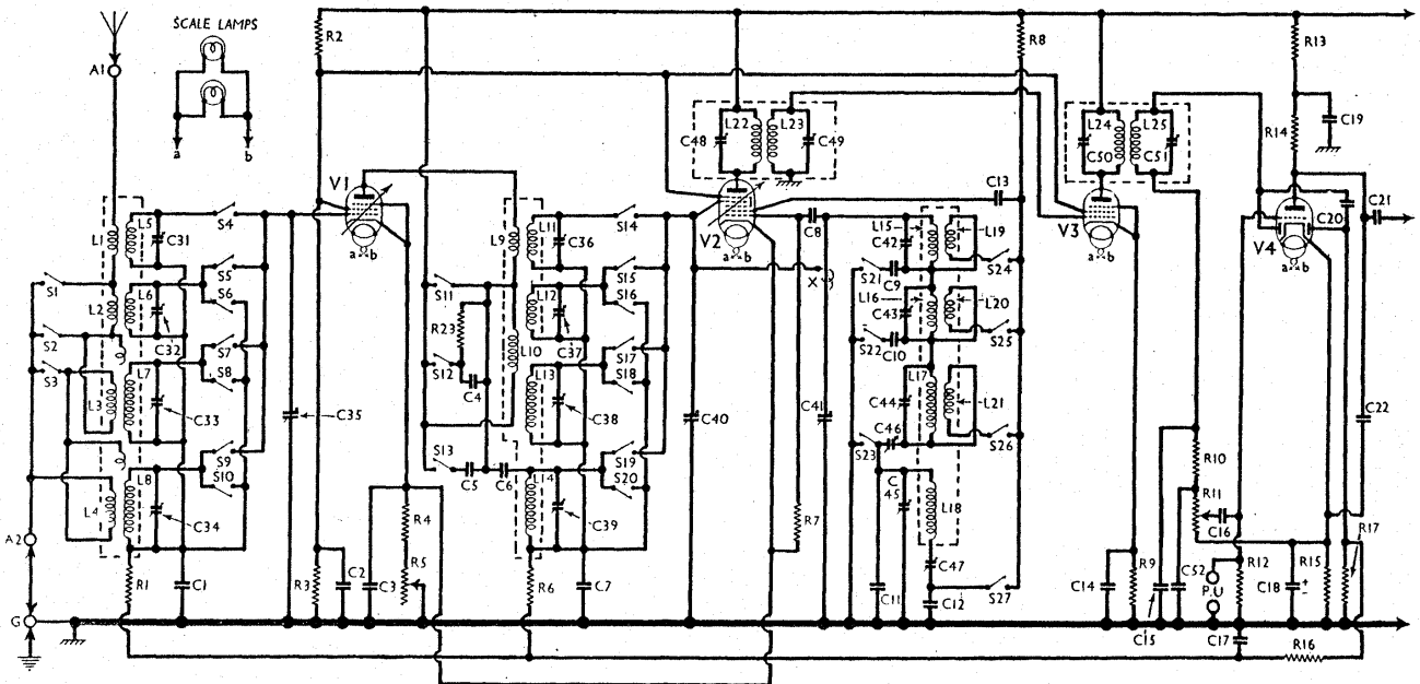
Circuit diagram of the Ferguson Model 350 all-wave A.C. superhet. The numbers in circles refer to the connections of the speaker plug and socket, a numbered diagram of which, viewed from the free ends of the pins, is inset in the extension of the diagram on the opposite page.
